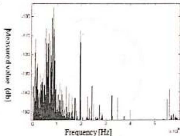
Fig. 1. Measurement of Spectrum utilization at BWRC
