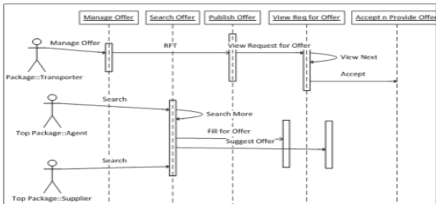
Fig: Sequence Diagram for Offer Service in ETransQ
