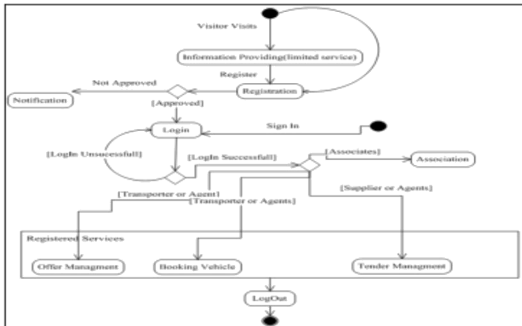
Fig: State Chart Diagram for ETransQ System
