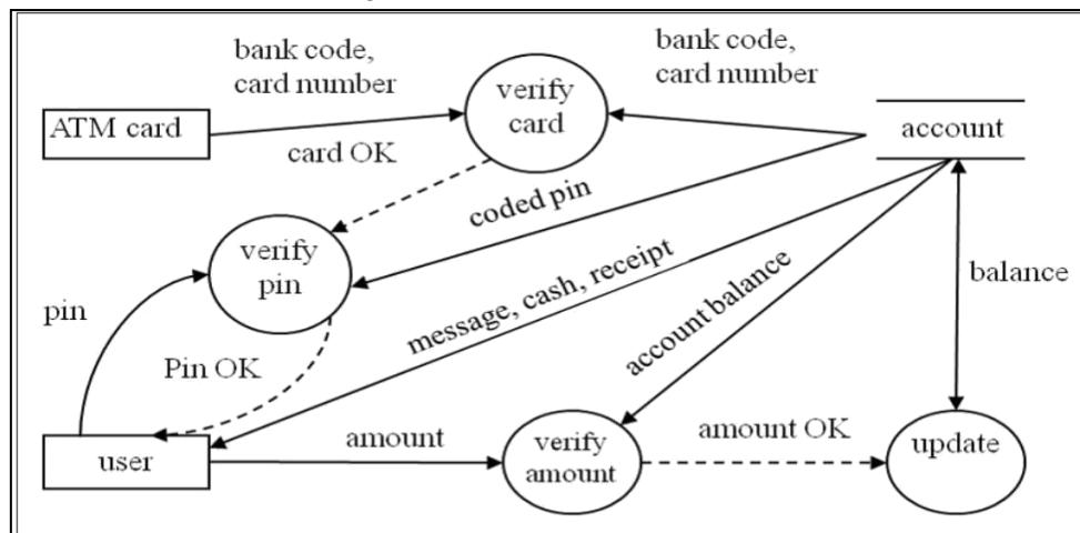
Fig: DFD for ATM Withdrawal
