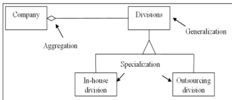
Fig: Aggregation, Generalization and Specialization
