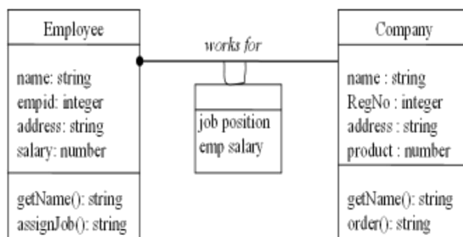
Fig: Class Diagram and Association of an Employee in a Company
