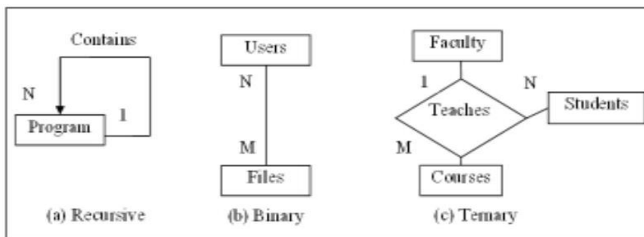
Fig: Relationships with Cardinalities
