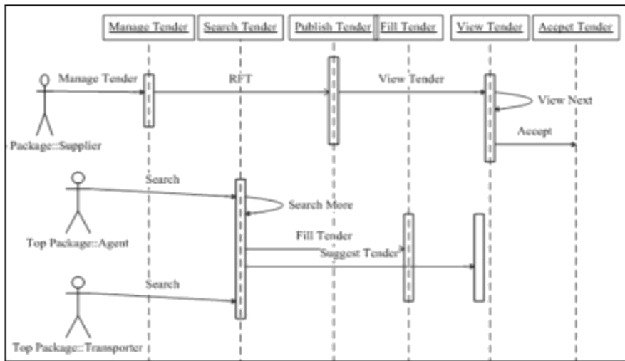
Fig: Sequence Diagram for Tender Service in ETransQ
