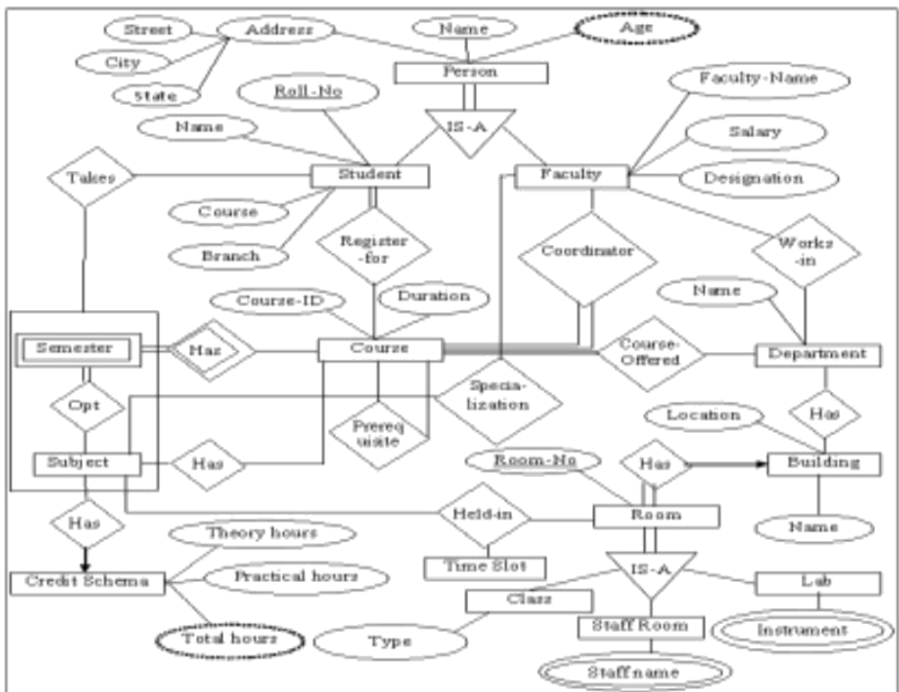
Fig: ER Diagram for Course Registration
