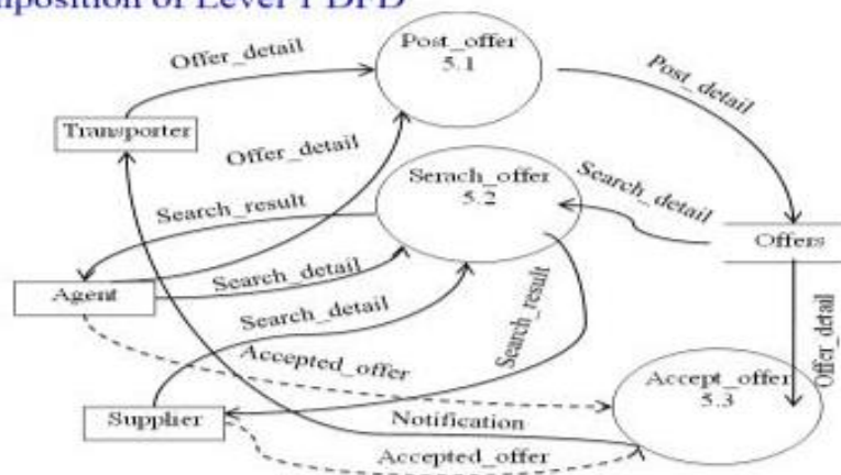
Fig: Level-2 DFD for Tenders in ETransQ
