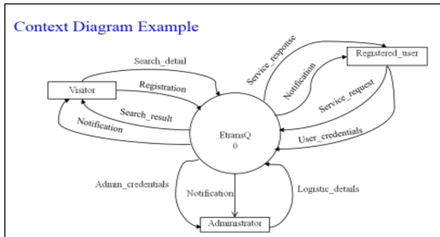
Fig: DFD – 0 for ETransQ System
