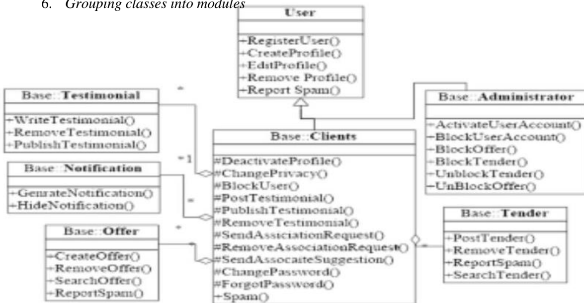
Fig: Class Diagram for ETransQ System
